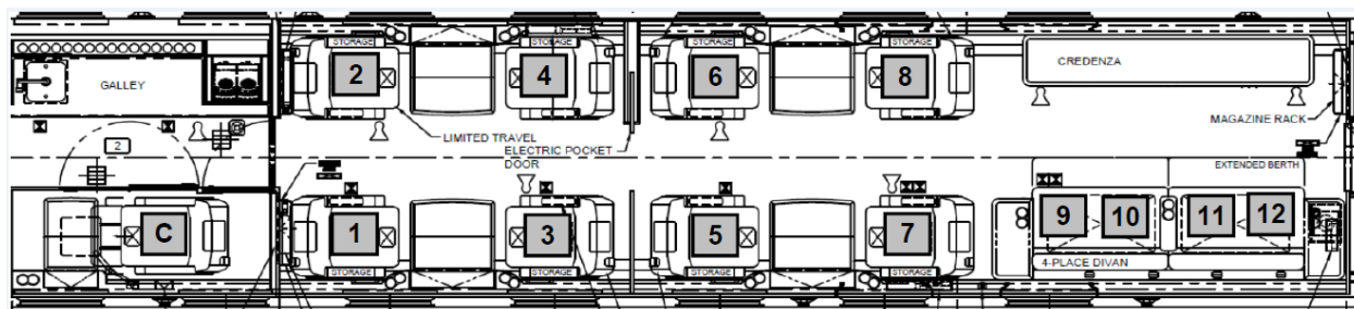
Floor Plan
